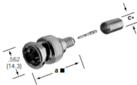
75Ω BNC Crimp Plugs
