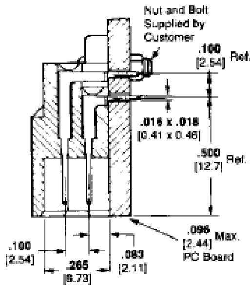
Standard Housing
