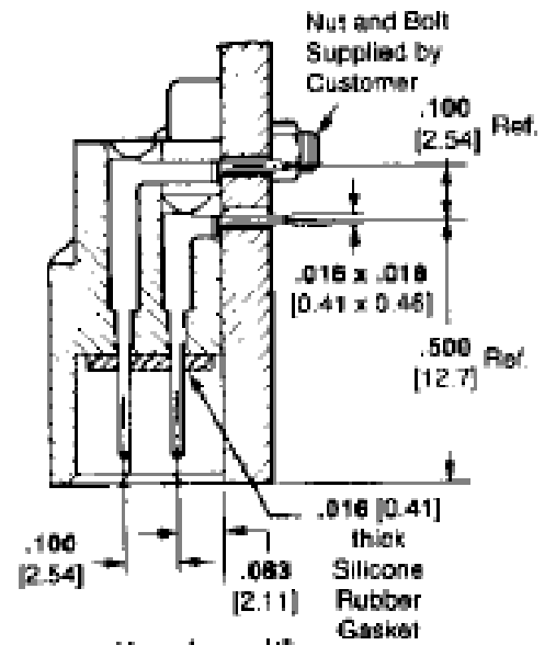
Housing with Interfacial Gasket
